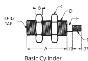
Basic Cylinder
