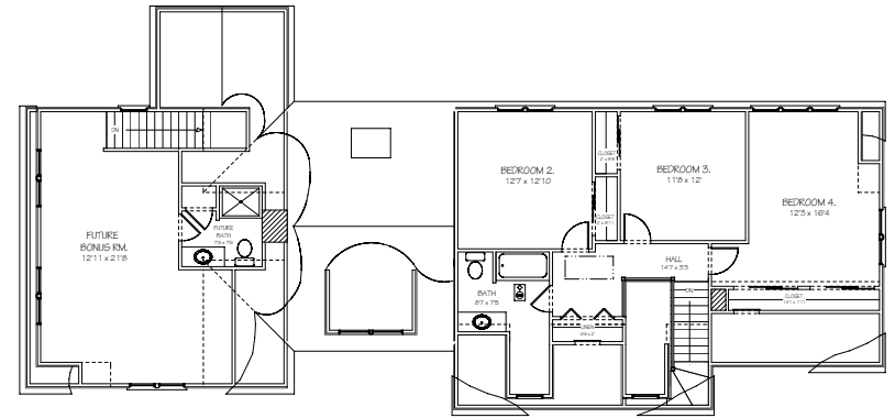
▲ Second Floor Plan - 803 S.F. Liv. Area
