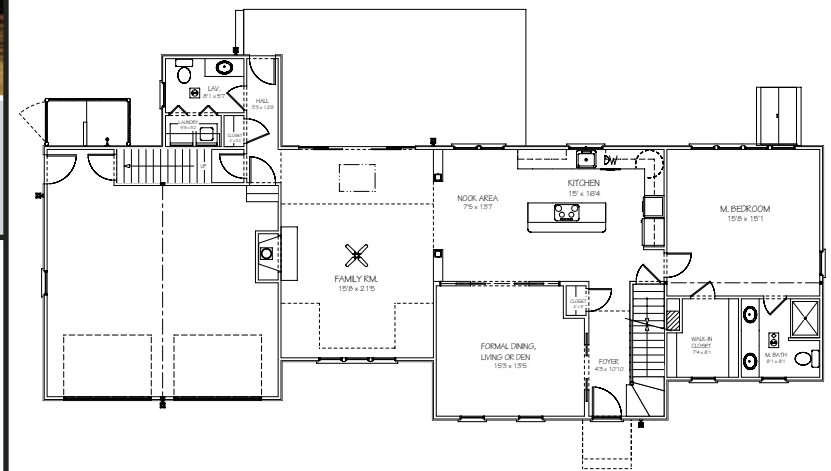
▼ First Floor Plan - 1,537 S.F. Liv. Area
