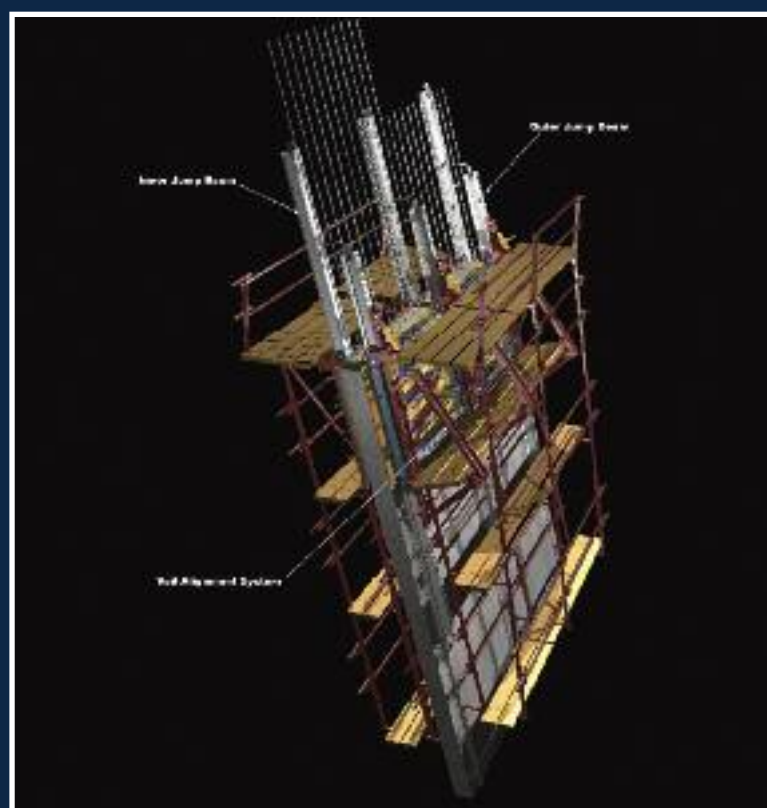
TYPICAL ASSEMBLY
