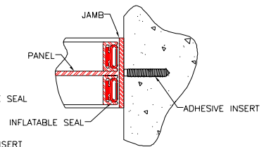
STANDARD JAMB MOUNT SECTION C-C
