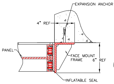
ALTERNATE FACE MOUNT SECTION A-A
