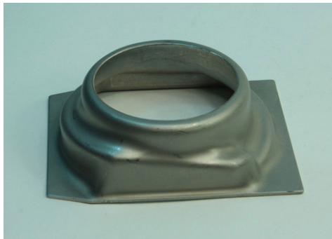
14 gauge 304 s/s spring retainer 5” square X 1.625” height made on a hydroform press.
