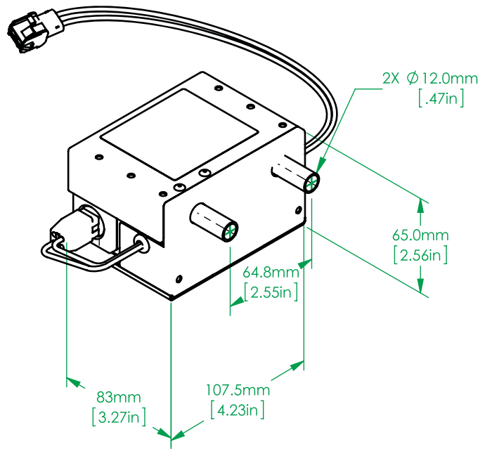
Power Supply
