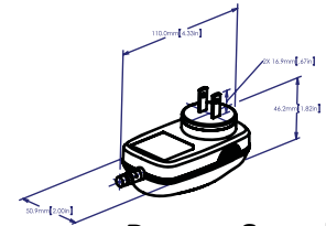
Power Supply
