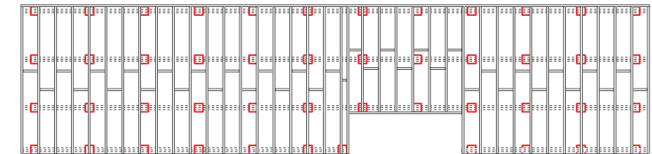
Fig 1.2: Traditional timber deck structure
