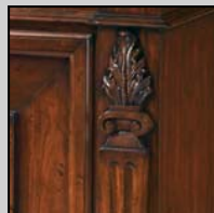
Intricate carvings
