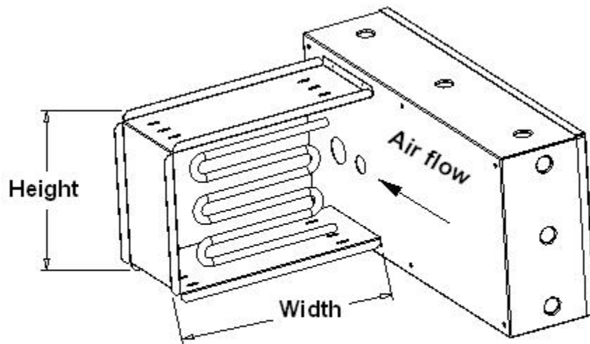
Horizontal Duct System Shown
