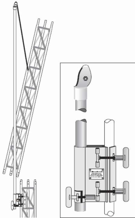
Erection Fixture: 2.5 in. sheave with 3/8 in. ID groove. For lifting tower sections during installations
