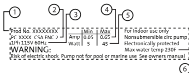
Fig. 6 Nameplate
