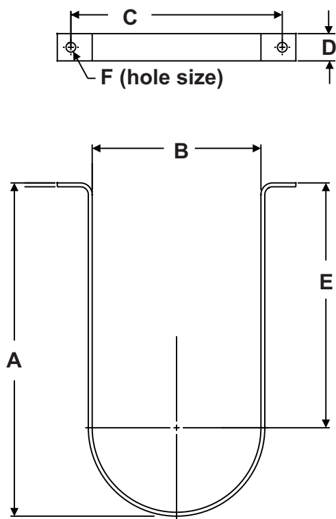
Figure 1. 4070-cu. in. Combined Cylinder Strap (P/N 06-236173-001)
