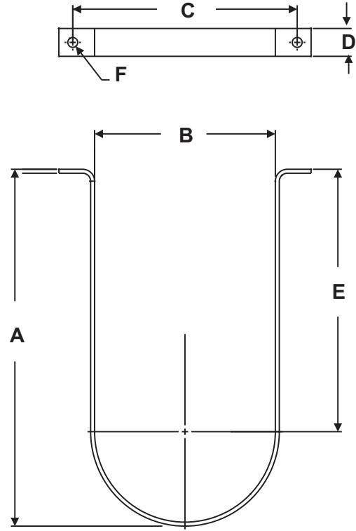
Figure 2. 4890-cu. in. Combined Cylinder Strap (P/N 06-236173-001)
