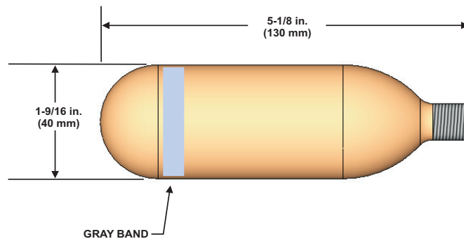
Figure 2. System Nitrogen Cartridge, P/N 87-120043-001
