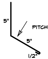
10 SIDEWALL
