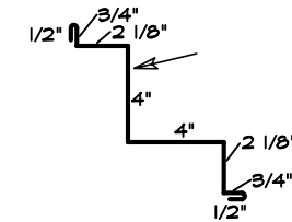
15 OUTSIDE CORNER
