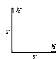
19 F TRIM FOR SOFFIT
