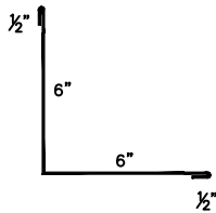
14 INSIDE CORNER
