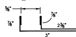
17 24" W-VALLEY
