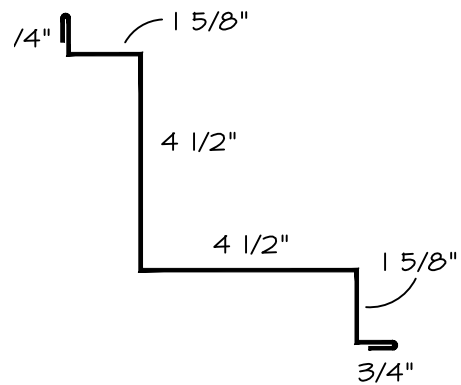
Inside Corner 10'-2" Pcs.
