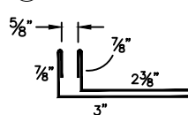
17 24" W-VALLEY
