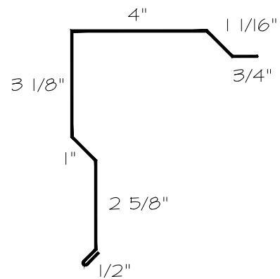
2x6 Gable
