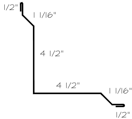
Inside Corner
