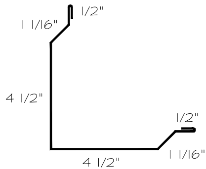
Outside Corner
