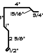
4a 2X6 GABLE
