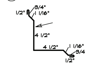
15 OUTSIDE CORNER
