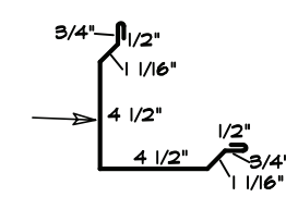
16 BASE TRIM
