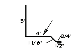
11 SNOW BREAK
