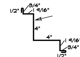
14 INSIDE CORNER
