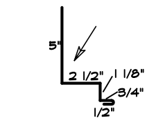
11 SNOW BREAK
