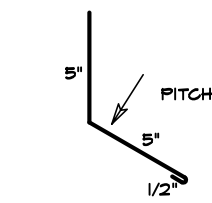
10 SIDEWALL
