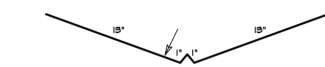
17 28" W-VALLEY
