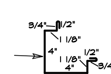
15 OUTSIDE CORNER
