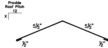
2 HIP RIDGE
