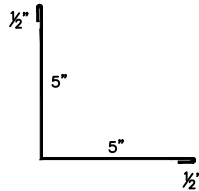
14 INSIDE CORNER
