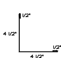
15) OUTSIDE CORNER
