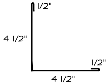
Outside Corner 10'-2" Pes.
