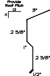
20a) TRANSITION HIGH LOW
