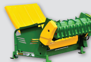
Chainless X25000 • 3pt mounted, self-loading • 1 bale capacity • Up to 5 ft wide bales
