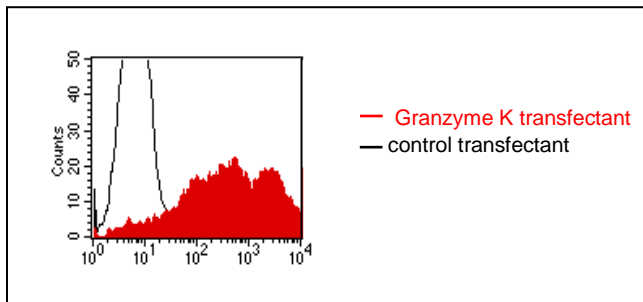
Fig.1: FACS analysis of BOSC23 cells using GM-6C3 Cat.# GM-0205. BOSC23 cells were transiently transfected with an expression vector encoding either Granzyme K (red curve) or an irrelevant protein (control transfectant: black curve). Binding of GM-6C3 was detected with a PE-conjugated secondary antibody. A positive signal was obtained only with Granzyme K transfected cells.
