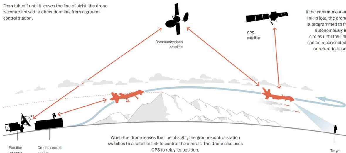
Figure 3: Typical Wireless Communication System for Military UAVs [4]
