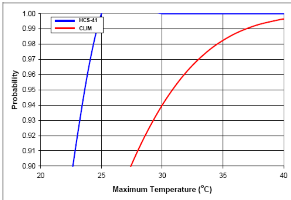
Figure 3: A magnification of the probability distribution from Figure 2
