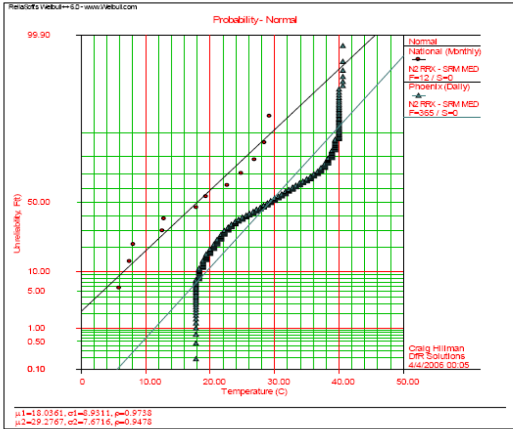
Figure 1: Distributions for daily maximum temperatures in Phoenix, AZ (green triangles) and monthly maximum temperatures from an average of 275 American cities (red circles)
