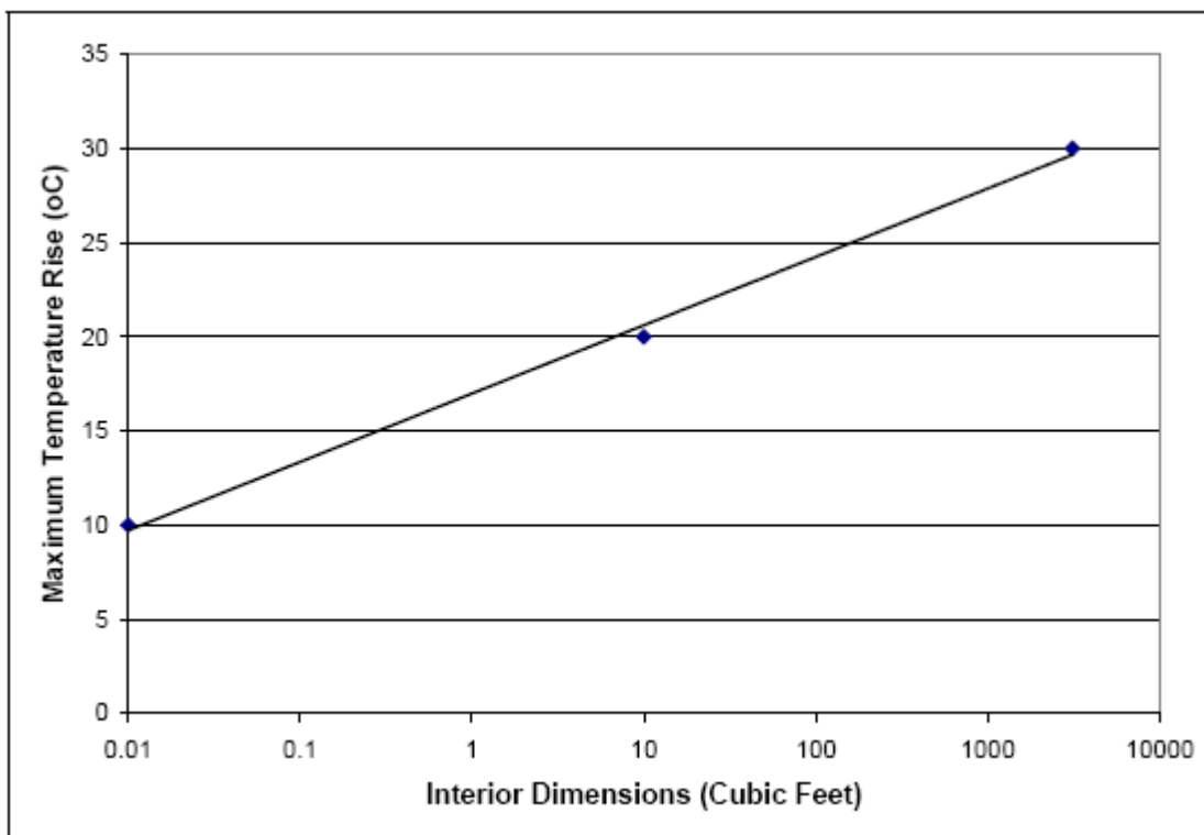
Figure 4: Maximum temperature rise at approximately 35C outdoor temperatures
