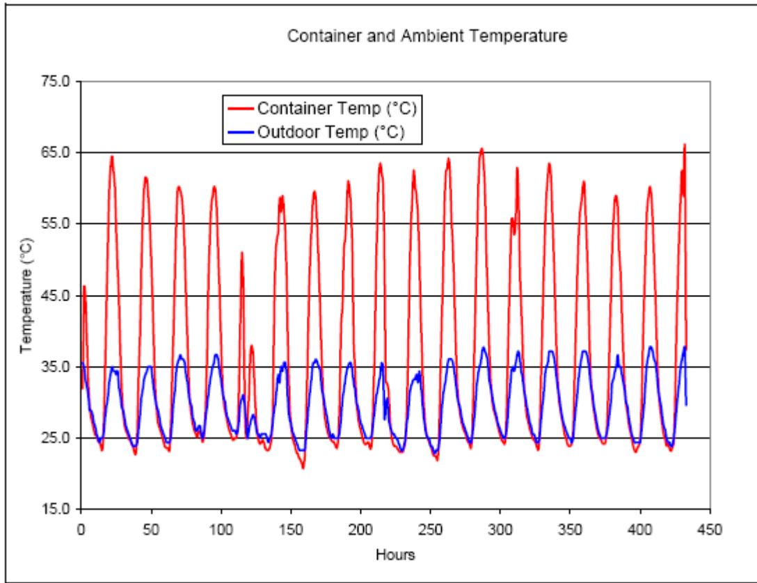
Figure 5: Variation in shipping container temperature as a function of outdoor air temperatures
