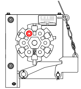
Tension Headplate Detail
