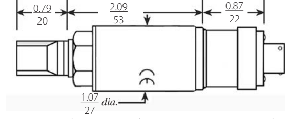
Shown w/10-6 Bayonet Connector and 1/4-18 NPT Pressure Fitting
