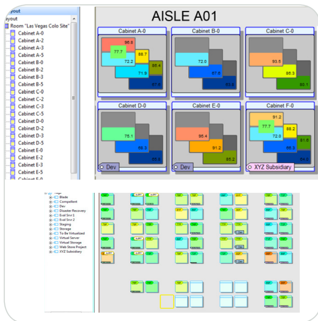
▶ Real time environmental data results in detailed facility wide images that show temperature down intra rack resolution using 3D heat maps
