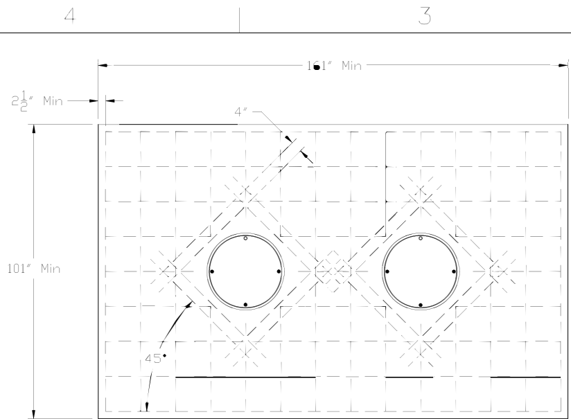
CONCRETE SLAB DETAIL FOR H20/HS20 LOAD RATING
