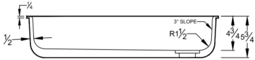
SECTION VIEW
