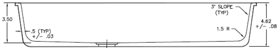
FRONT VIEW
