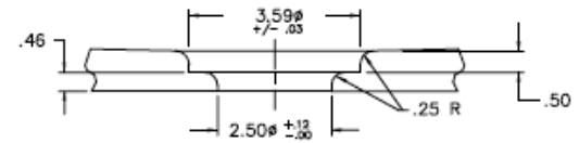
TO5 DRAIN OPENING DETAIL SECTION A-A
