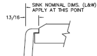
WALL DETAIL AT LIP
