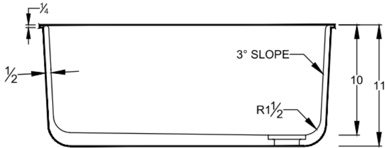
SECTION VIEW
