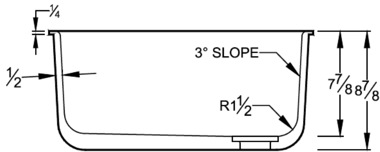
SECTION VIEW
