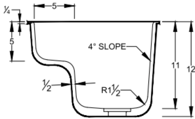
SECTION VIEW (FRONT TO BACK)
