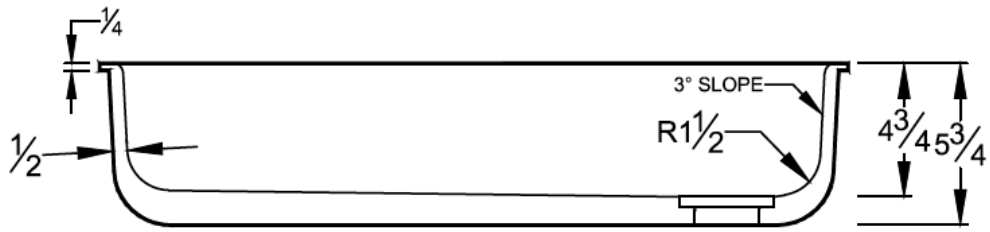
SECTION VIEW
