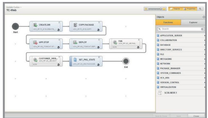
Integrated Workflow Editor
