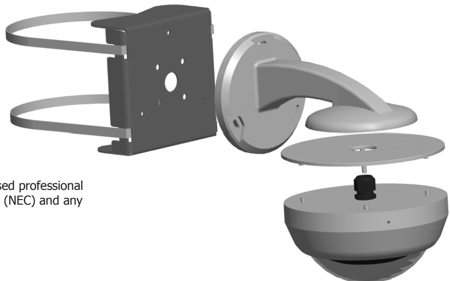
Figure 1 - BMT-75PM Exploded View with BMT-75WA and BDH-7500 Shown
