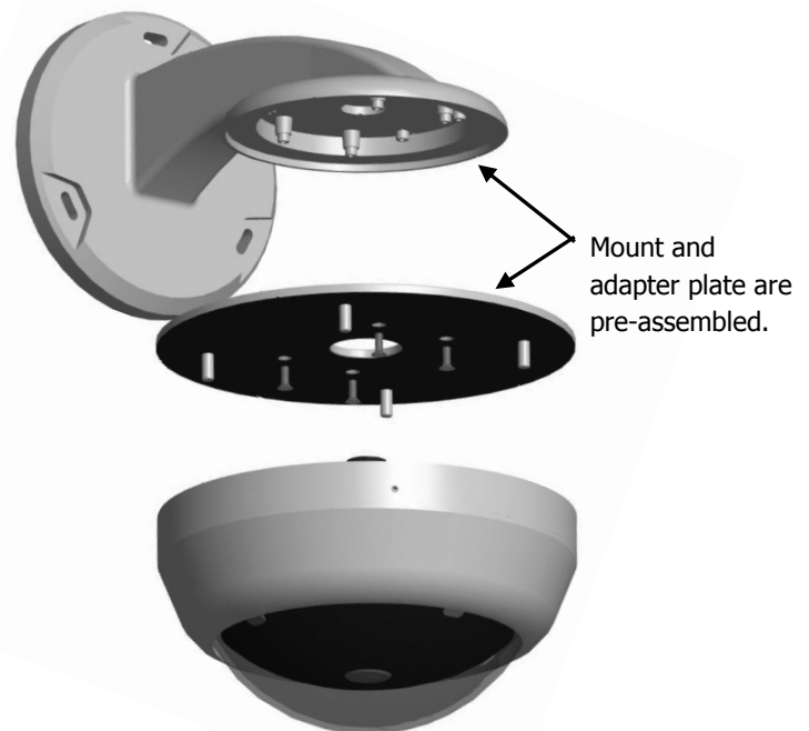
Figure 1 - BMT-75WA Exploded View with BDH-7500 Shown
