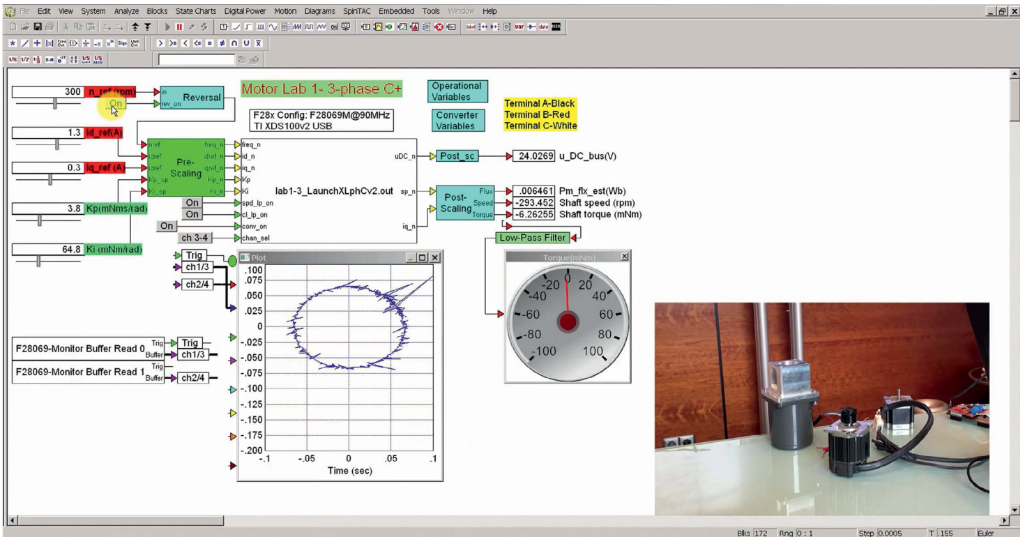
Hardware-in-the-Loop Set-up of a Field Oriented Control System
