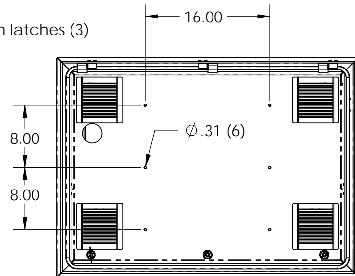
REAR VIEW (mounting pattern)
