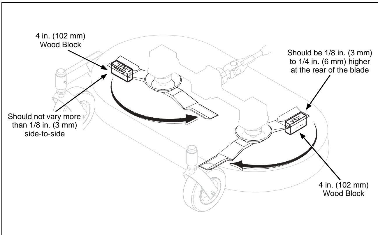
Deck Leveling
