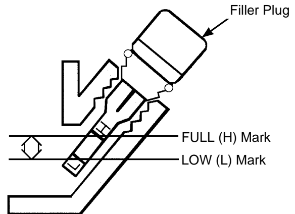
Dipstick Position for Checking Oil Level
