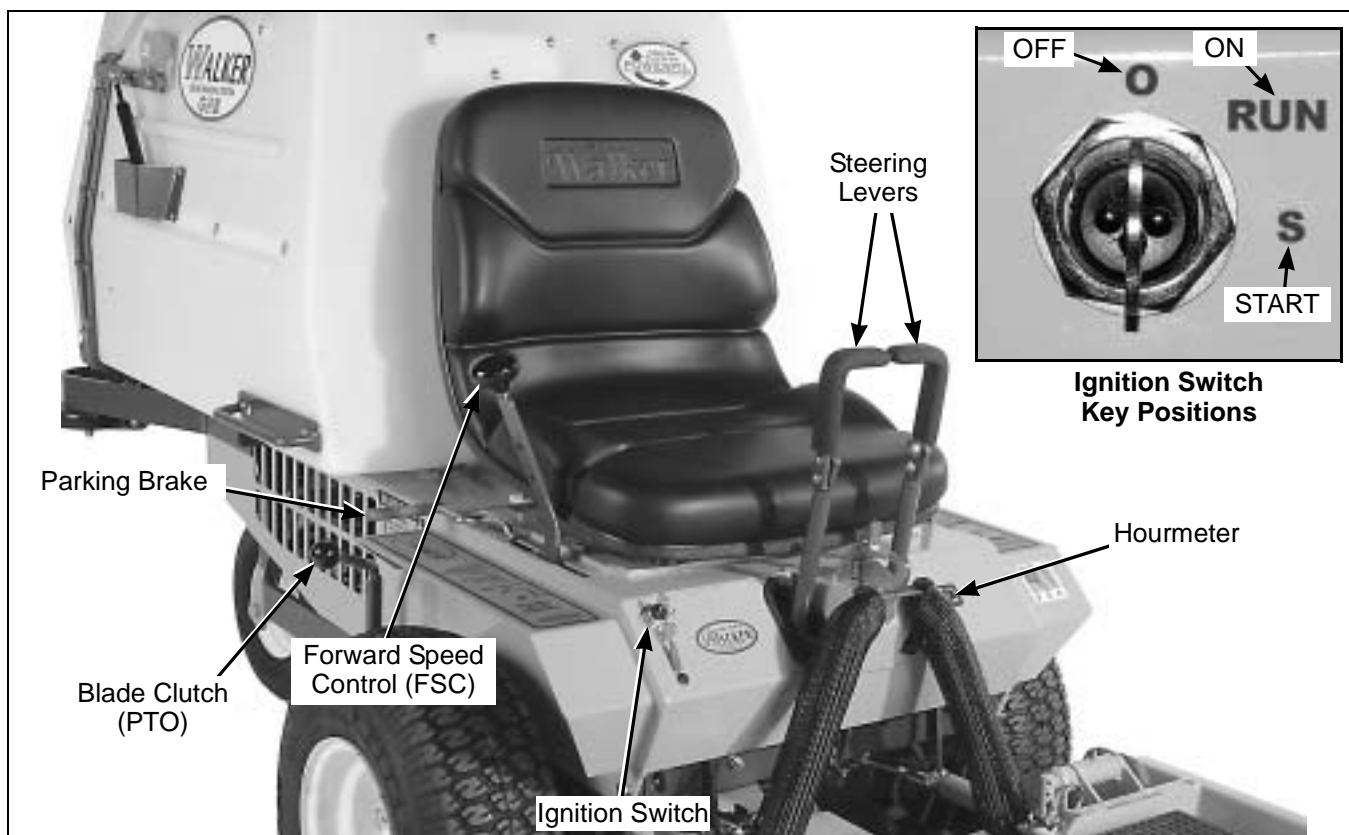
Operating Controls
