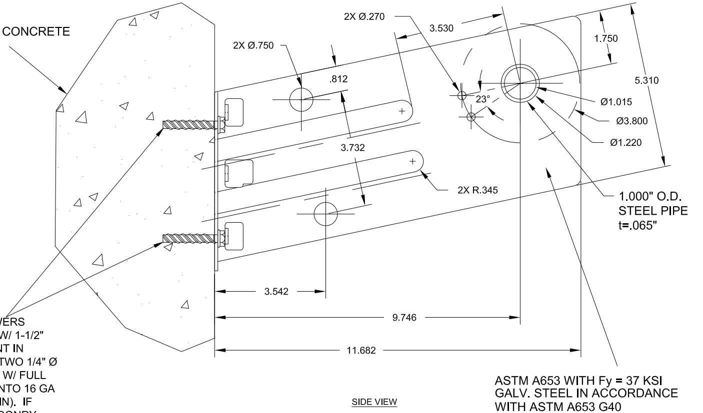
DOOR MOUNTING BRACKET DETAIL
