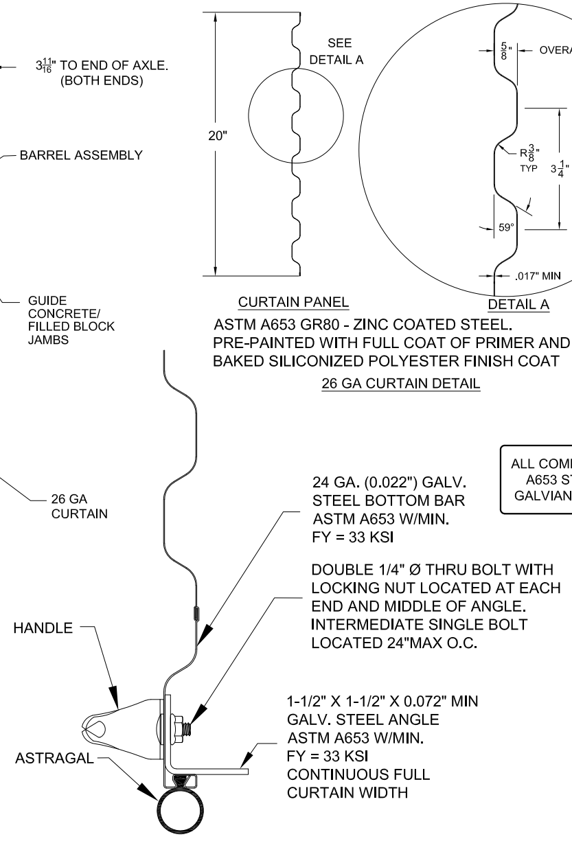
BOTTOM BAR ASSEMBLY
