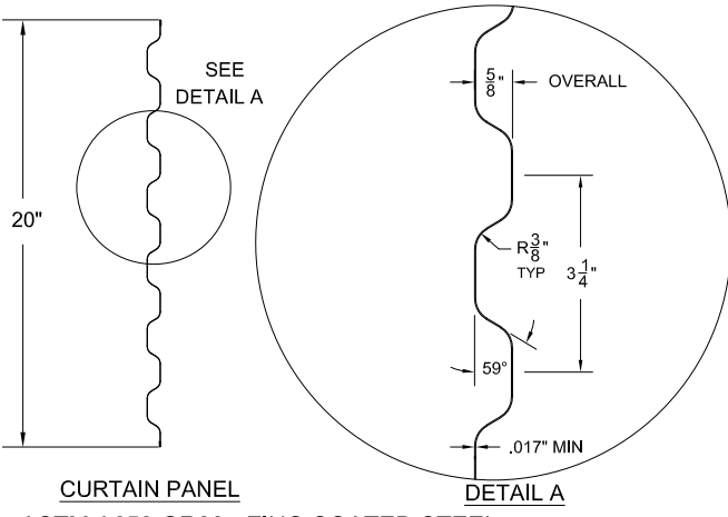
CURTAIN PANEL ASTM A653 GR80 - ZINC COATED STEEL. PRE-PAINTED WITH FULL COAT OF PRIMER AND BAKED SILICONIZED POLYESTER FINISH COAT 26 GA CURTAIN DETAIL
