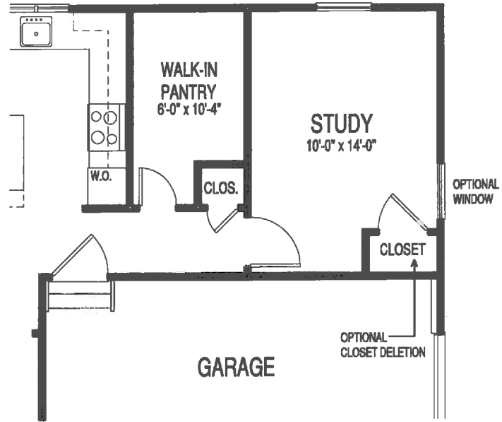
OPTIONAL STUDY WITH WALK-IN PANTRY (LAUNDRY RELOCATED TO SECOND FLOOR)
