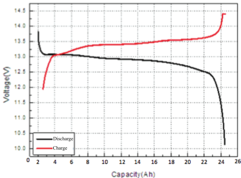
12.8V24Ah Charge-Discharge C 5 ,25°C
