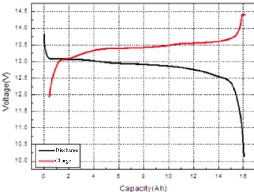
12.8V16Ah Charge-Discharge C 5 ,25°C
