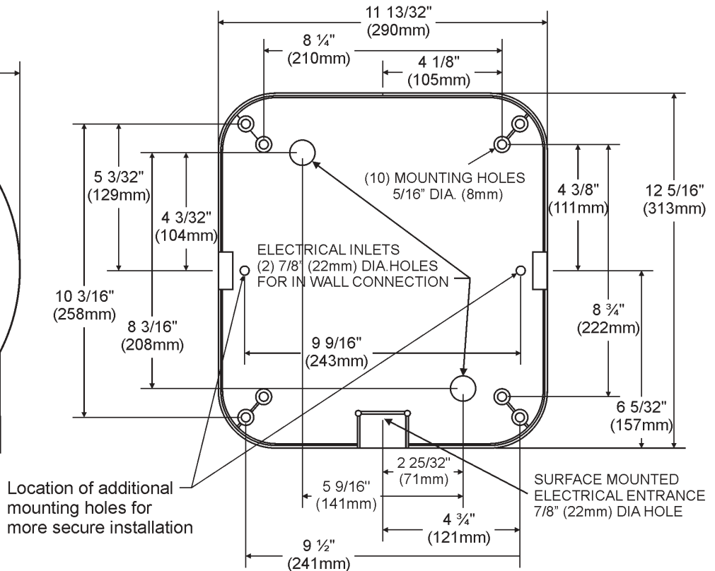
FRONT VIEW FACING WALL
