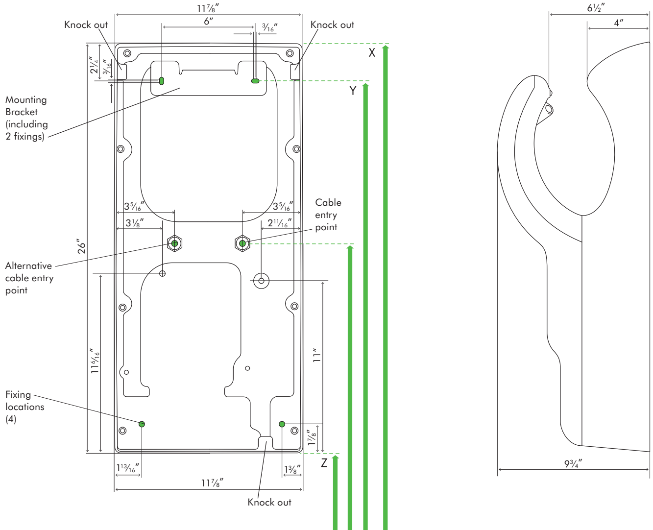
REAR ELEVATION
